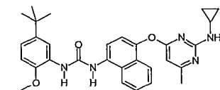
1-(5-tert-Butyl-2-methoxy-phenyl)-3-[4-(2-cyclopropylamino-6-methyl-pyrimidin-4-yloxy)-naphthalen-1-yl]-urea;
